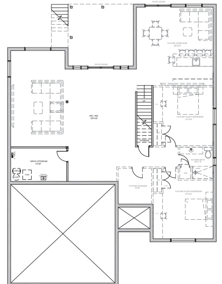
BASEMENT PLAN
