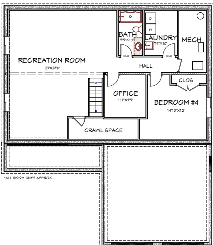
BASEMENT PLAN
