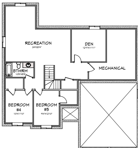
BASEMENT PLAN
