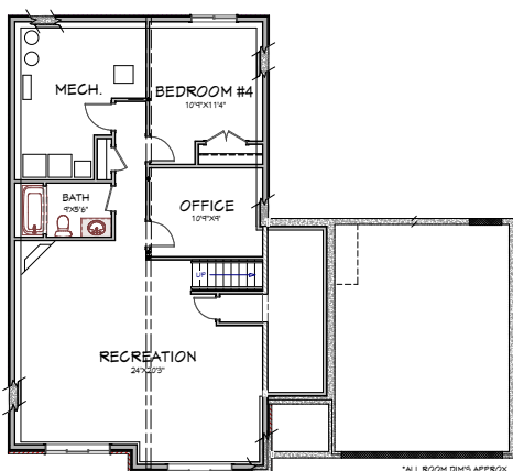
BASEMENT PLAN
