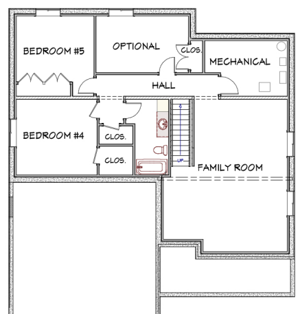
BASEMENT PLAN
